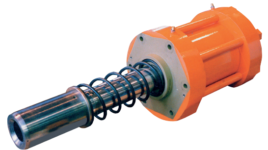
Subsea Collet Cylinder
